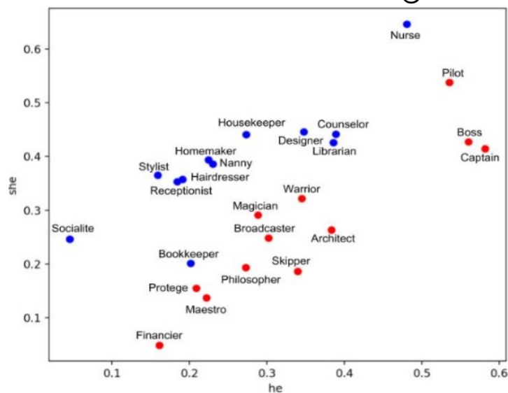
Word Embedding
